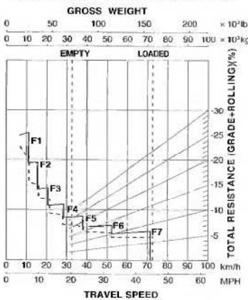
HD605 Grade distance: 900 m (2950 ft)
