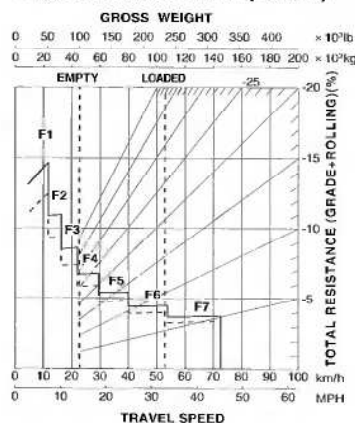
HD605 Grade distance: 900 m (2950 ft)
