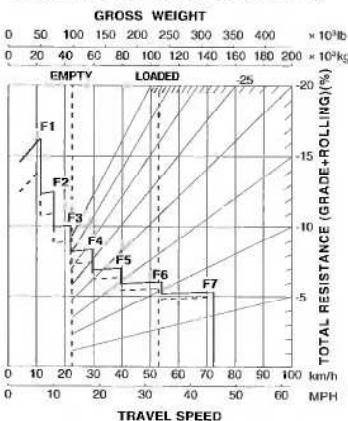
HD605 Grade distance: 450 m (1480 ft)
